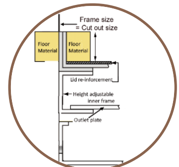
Retro base assembly
