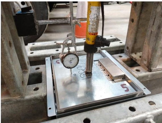
Photo 1 – View of testing arrangements
