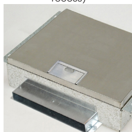
Spigot for in screed trunking (trimless shown)
