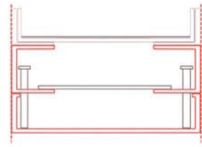
Retrofit floor box without fixing flange (floor box installed AFTER final floor is fitted or with a poured finish, i.e. terrazzo/polished screed)
