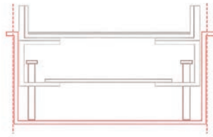
Standard floor box with fixing flange (base box installed BEFORE final floor is fitted)
